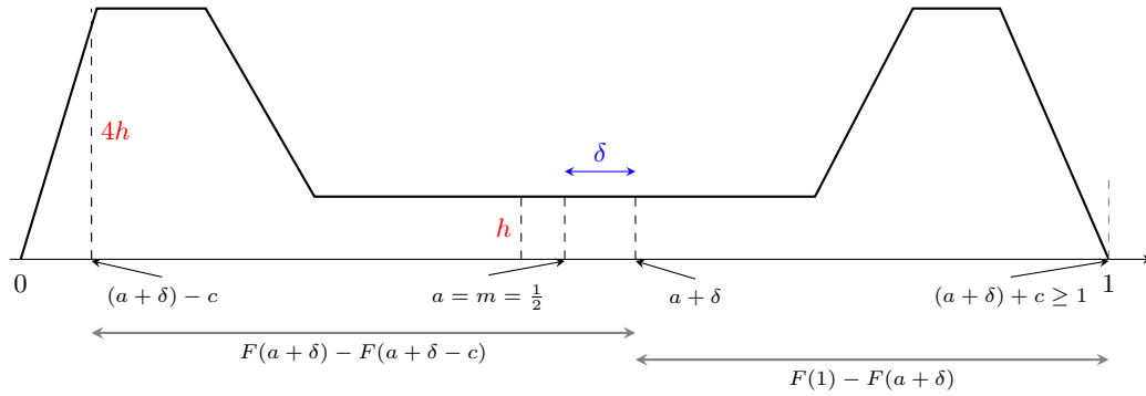
Fig. 2. A schematic density for which the ordinary median m = 1/2 is a c -conditional median, but another point a + \delta \neq m is also a c -conditional median. Here c = 1/2 , so the window around a + \delta is truncated at the right endpoint.
