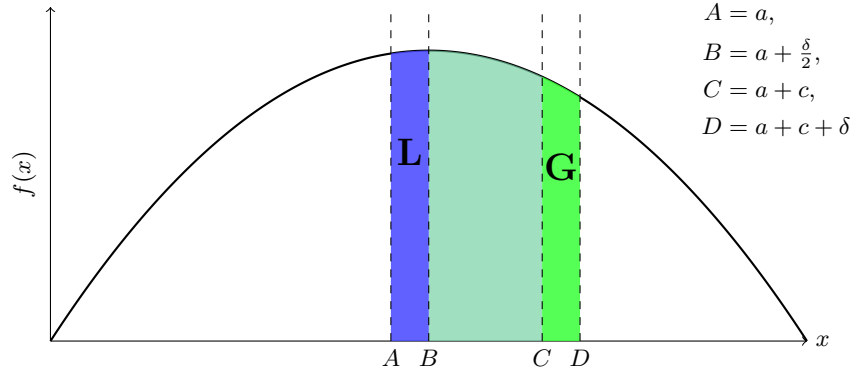
Fig. 3. Local deviation at the conditional median a . The blue window represents the original attraction interval [a, a + c] , while the green window represents the shifted interval [a + \frac{\delta}{2}, a + \delta + c] . Their overlap is shaded naturally. Mass L lost near the center is counted twice in the vote-share margin, whereas mass G gained at the boundary is counted once.
