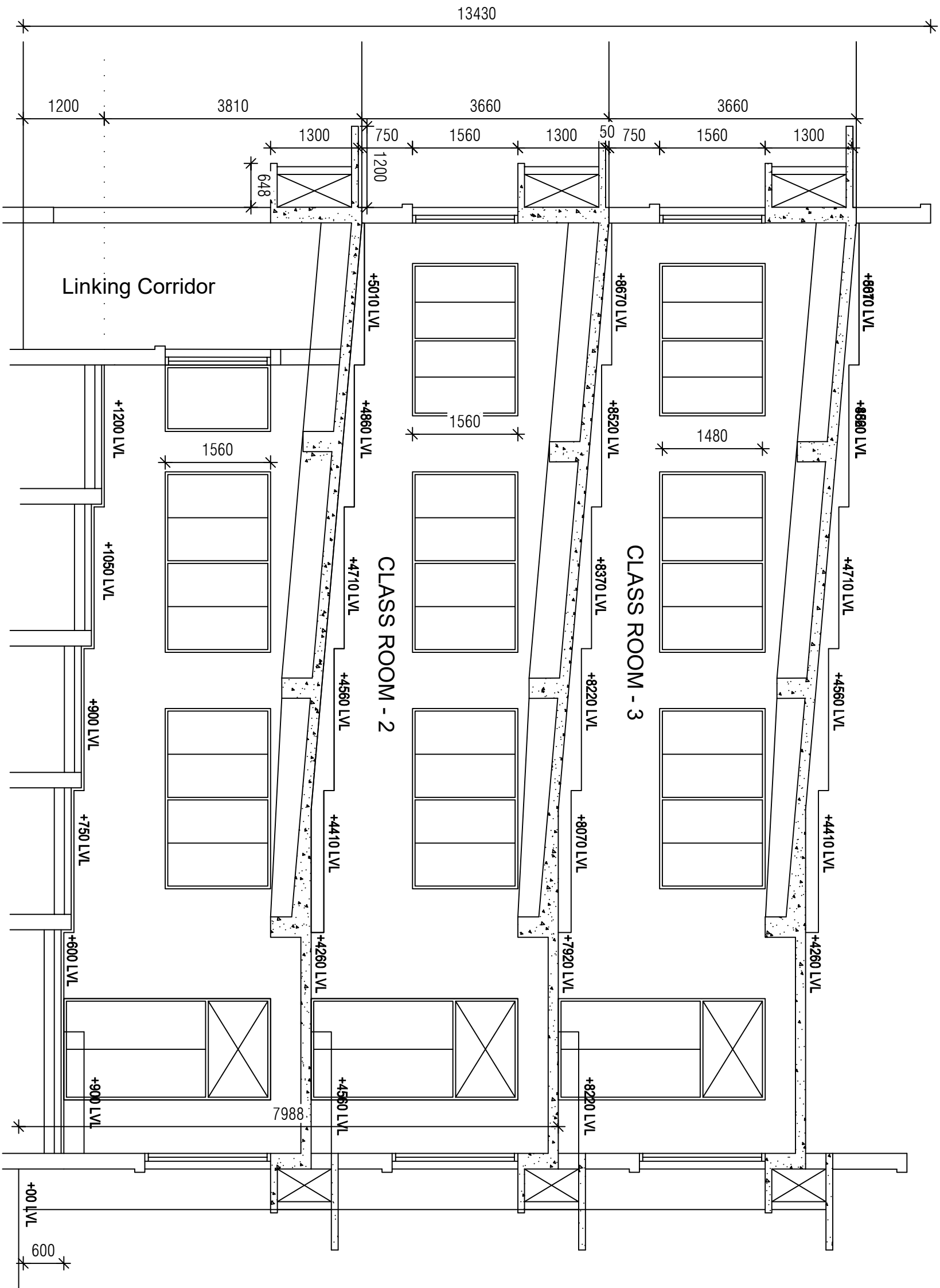
Section - AA
